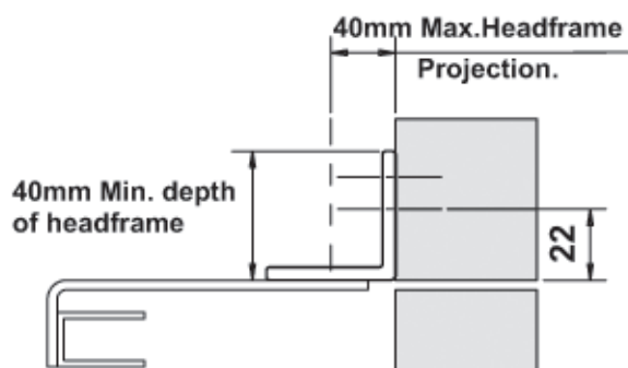
FIG.38 APPLICATION FOR HEAD PROJECTION OF LESS THAN 44mm.
